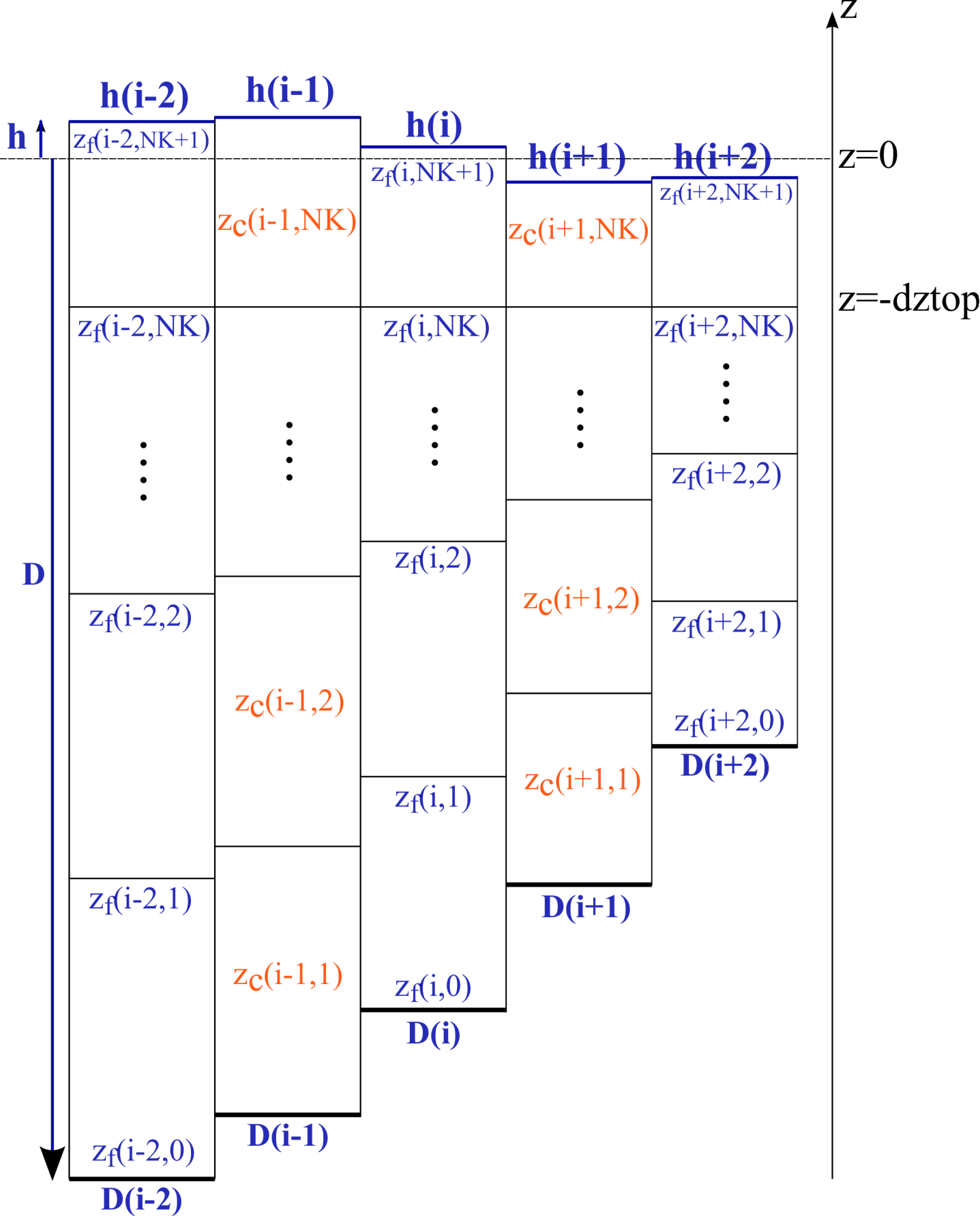
2D view of the vertical grid.
